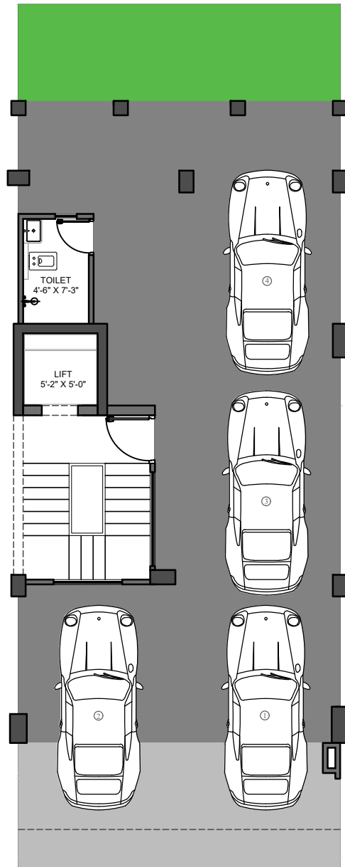
STILT FLOOR PLAN
