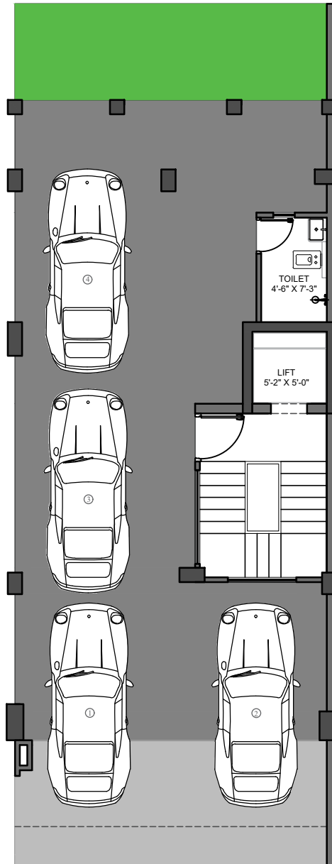
STILT FLOOR PLAN
